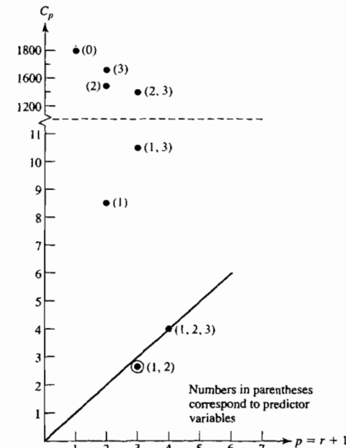
Figure 7.4 C_p plot for computer data from Example 7.6 with three predictor variables ( z_1 = orders, z_2 = add-delete count, z_3 = number of items; see the example and original source).
