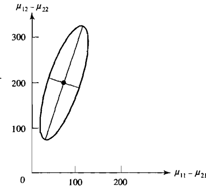
Figure 6.2 95% confidence ellipse for \boldsymbol{\mu}'_1 - \boldsymbol{\mu}'_2 = (\mu_{11} - \mu_{21}, \mu_{12} - \mu_{22}) .
