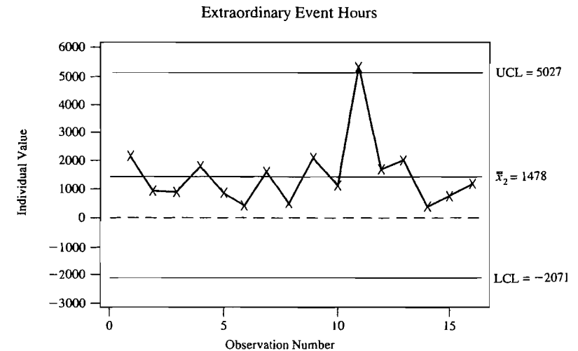
Figure 5.7 The \bar{X} -chart for x_2 = extraordinary event hours.
