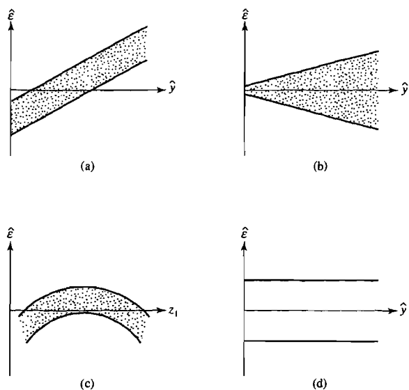
Figure 7.2 Residual plots.
